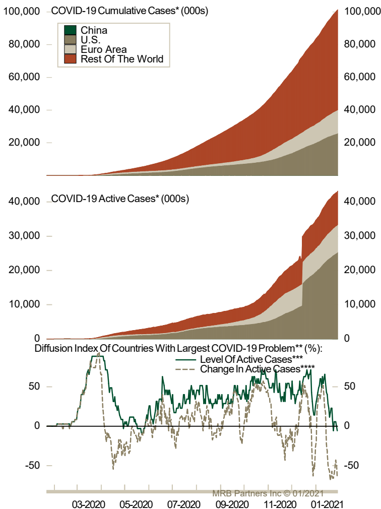
The Global COVID-19 Curve
